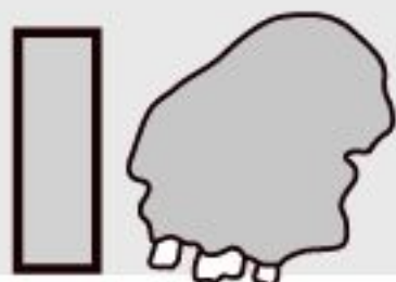
Kenyanthropus platyops
